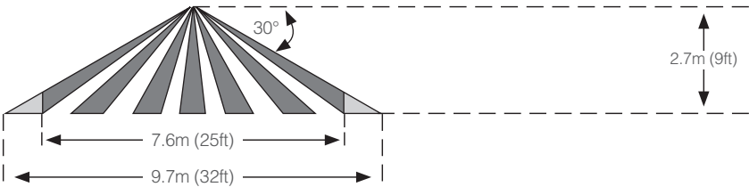
PIR Area of Detection (Side View)
