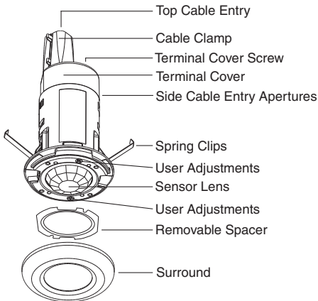
753 SERIES SENSOR
